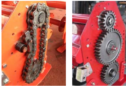
Heavy Duty 16A Side Chain Drive or Gear Drive
